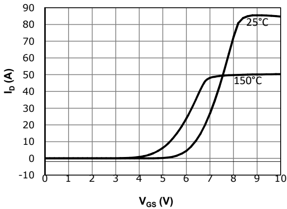
Fig 3: Transfer Characteristics
