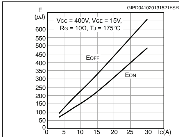
Figure 20. Switching-off loss vs collector current
