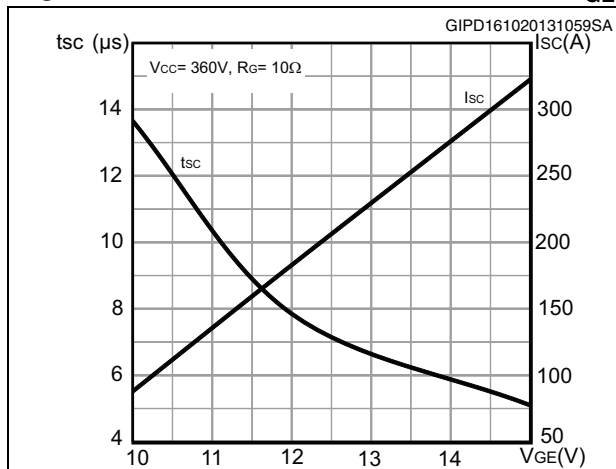
Figure 24. Short circuit time and current vs V GE
