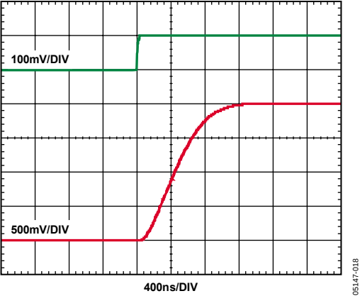
Figure 10. Rise Time
