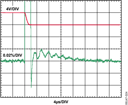
Figure 13. Settling Time (Falling)
