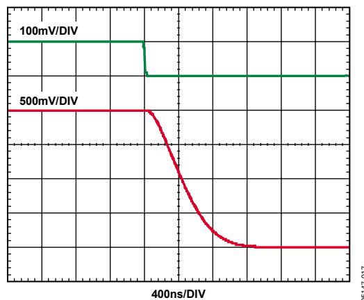
Figure 9. Fall Time
