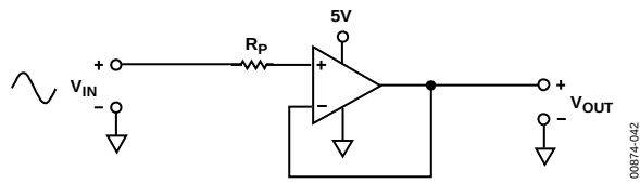
Figure 42. (a) Response with R_P = 0 ; V_{IN} from 0 V to +V_S (b) V_{IN} = 0 \text{ V to } +V_S + 200 \text{ mV} V_{OUT} = 0 \text{ V to } +V_S R_P = 49.9 \text{ k}\Omega
