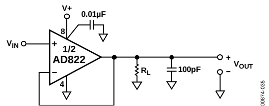
Figure 35. Unity-Gain Follower
