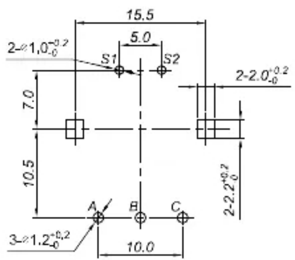
P.C.B. mounting hole detail
