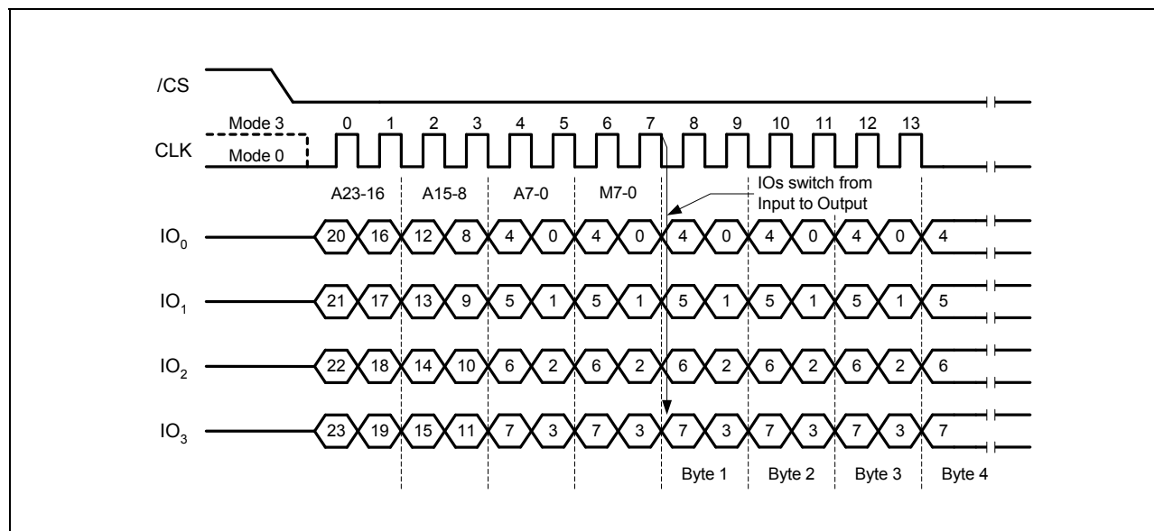
Figure 16b. Octal Word Read Quad I/O Instruction Sequence (Previous instruction set M5-4 = 10)
